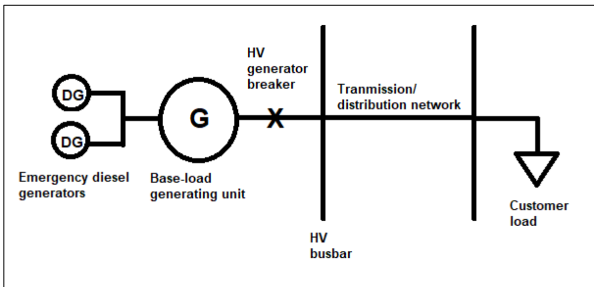
Figure 3 - Example of a full black-start test network for a base-load black-start facility
